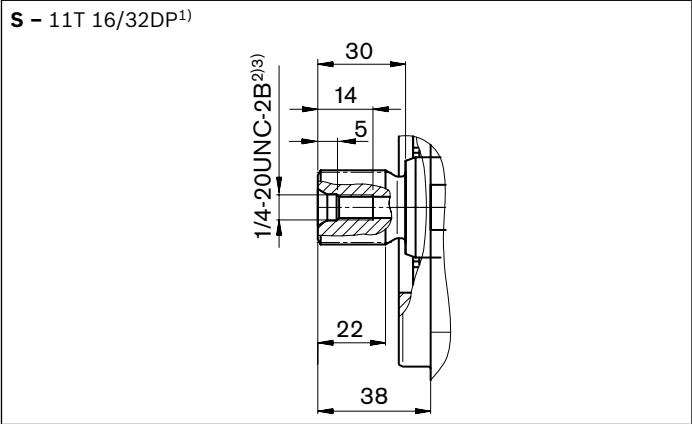
Connection table A10VZO
